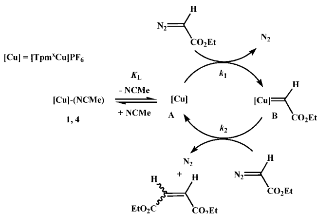
Scheme 4. Catalytic Cycle for the EDA Decomposition Reaction in the Presence of 1 or 4 as the Catalyst
