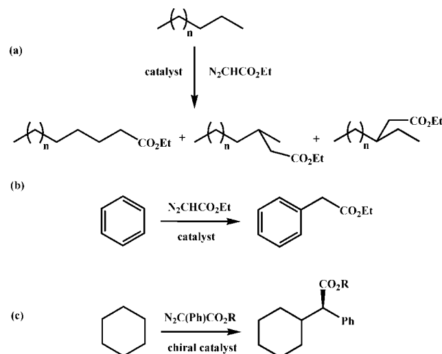
Scheme 1. Examples of the Catalytic Functionalization of Hydrocarbons by Carbene Insertion from Diazo Compounds
