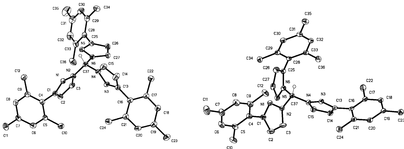
Figure 2. Molecular structures of (left) tris(3-mesitylpyrazol-1-yl)methane ( \text{Tpm}^{\text{Ms}} , 2 ) and (right) bis(3-mesitylpyrazol-1-yl)(5-mesityl-1-pyrazol-1-yl)methane ( \text{Tpm}^{\text{Ms}*} , 3 ). Thermal ellipsoids are drawn at the 50% probability level. H atoms have been omitted for clarity.
