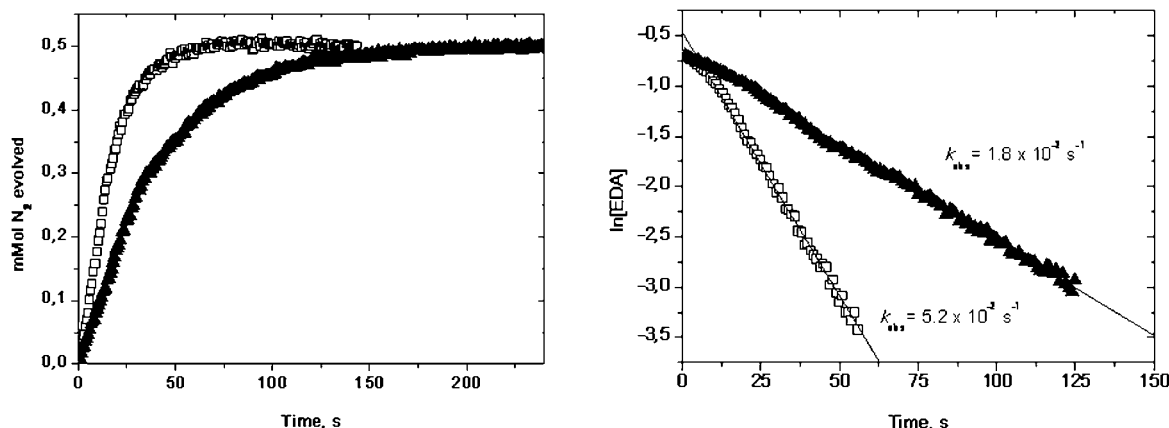
Figure 4. Plots of the evolution of N_2 and of \ln [EDA] vs time for the EDA decomposition using 1 (▲) and 4 (□) as the catalysts.
