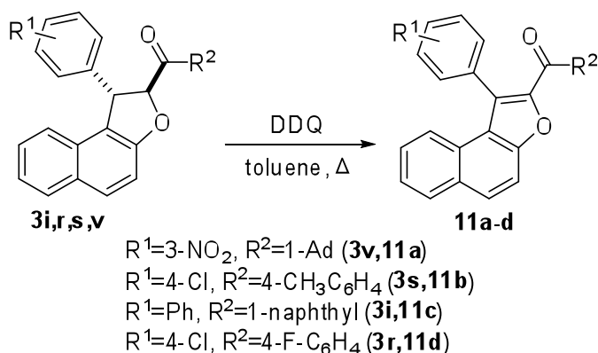
Scheme 9. Aromatization of 1,2-dihydronaphtho[2,1- b ]furans
