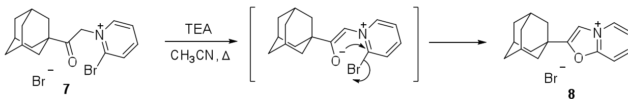
Scheme 7. Synthesis of oxazolo[3,2- a ]pyridinium salt 8
