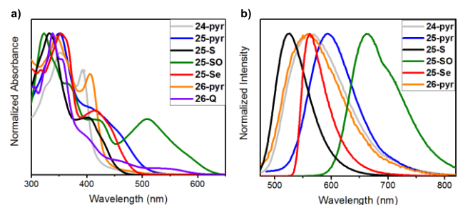
Figure 2. Normalized a) absorption and b) emission spectra ( CH_2Cl_2 ) for 24–26
