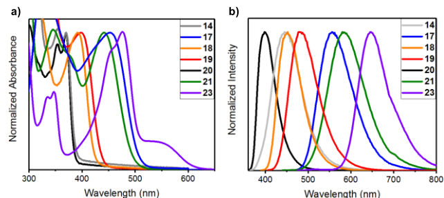
Figure 1. Normalized a) absorption and b) emission spectra ( CH_2Cl_2 ) for PAHs 14 , 17–21 , and 23 .
