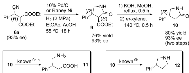
Scheme 1. Elaboration of Product 6a
