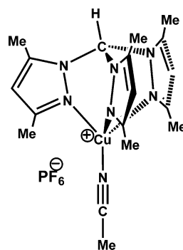
Figure 1. \{[\text{HC}(3,5\text{-Me}_2\text{pz})_3]\text{Cu}(\text{NCMe})\}\text{BF}_4 ( 1 ).
