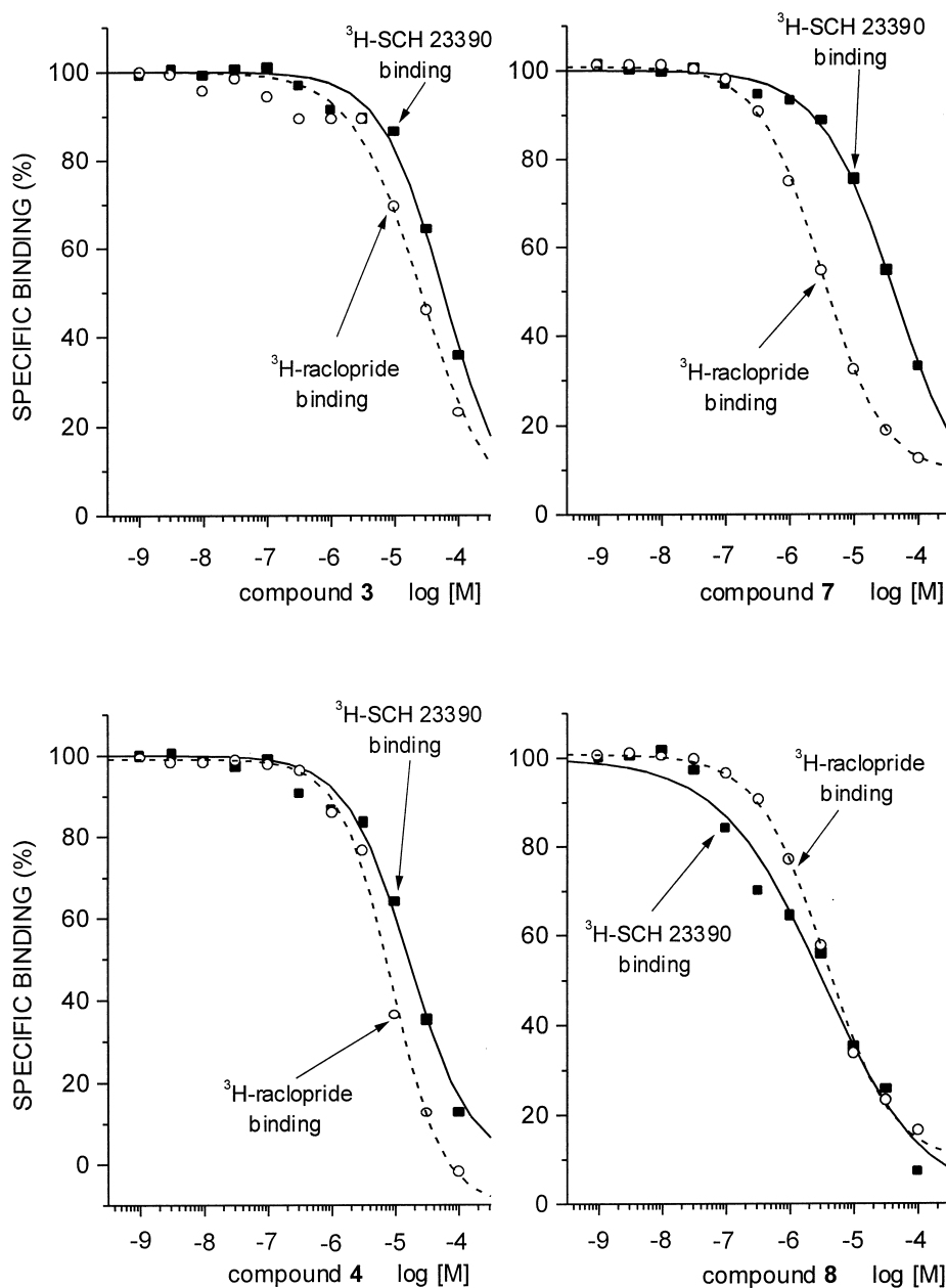
Figure 4. Comparative displacement curves of specific [ ^3 H]-SCH 23390 and [ ^3 H]-raclopride binding by BTHIQ compounds 3 and 7, and N -methyl-BTHIQ compounds 4 and 8. Displacement curves correspond to four determinations at each concentration.
