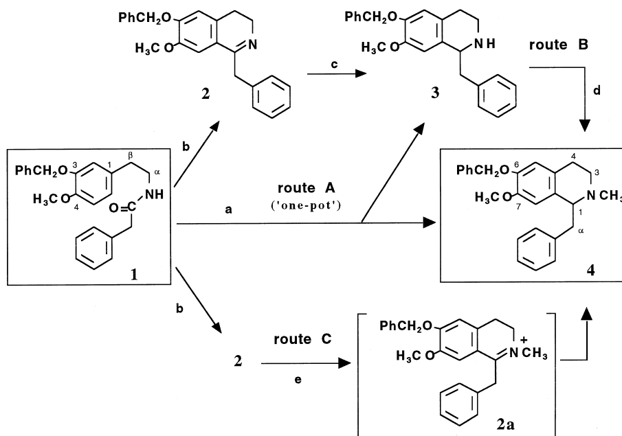
Figure 2. Syntheses of N -methyl-BTHIQ derivative 4 . Reagents and conditions: (a) POCl 3 /CH 2 Cl 2 , reflux, 3 h, followed by NaBH 4 /MeOH, −40 °C, 5 h; (b) POCl 3 /CH 2 Cl 2 , reflux, 3 h; (c) NaBH 4 /MeOH, rt, 2 h; (d) POCl 3 /MeOH, rt, 30 h; (e) POCl 3 /MeOH, reflux, 9 h, followed by NaBH 4 , rt, 3 h.
