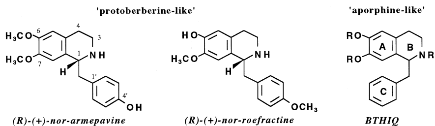
Figure 1. 1-Benzyl-1,2,3,4-tetrahydroisoquinoline analogues.
