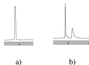
FIGURE 1. HPLC analysis using the chiral stationary phase: (a) racemic bis-epoxide (+/-)- 3 and (b) optically pure bis-epoxide (+)- 3 .
