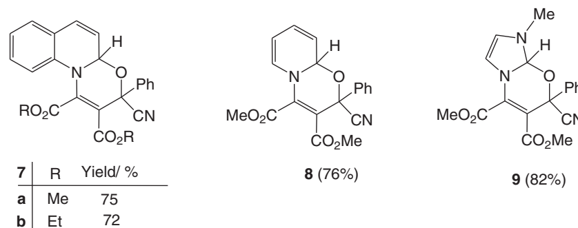
Scheme 3. Three-component reactions of benzoyl cyanide, activated acetylenes and quinoline, pyridine, and N -methylimidazole.
