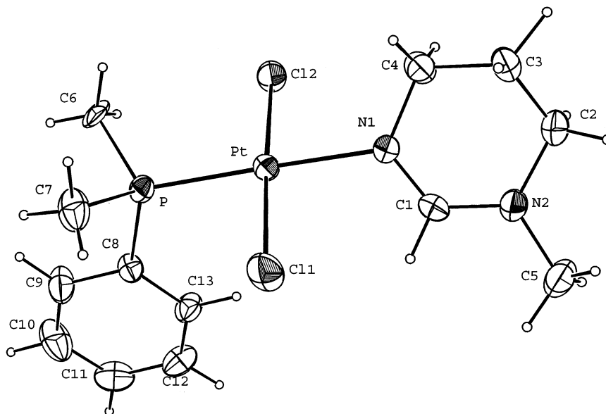
Fig. 2. ORTEP drawing of the structure of the trans -complex 2 , showing the atomic numbering scheme. Displacement ellipsoids of non-H atoms are shown at the 30% probability level and H atoms are drawn as small circles of arbitrary radii.
