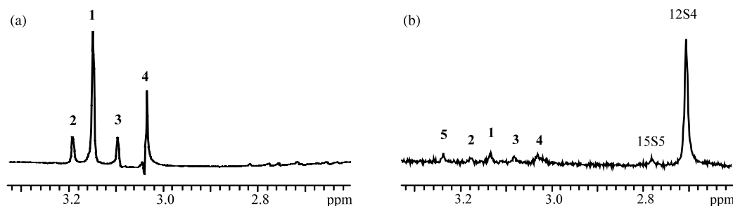
Fig. 1. (a) 1 H-NMR spectrum of the reaction of thiirane and Cr(NCCH 3 )(CO) 5 in the CH 2 region showing the resonances of the cyclic polydisulfides 1–4. (b) 1 H-NMR spectrum of the reaction of thiirane with Cr(NCCH 3 )(CO) 5 in the presence of DMAD.
