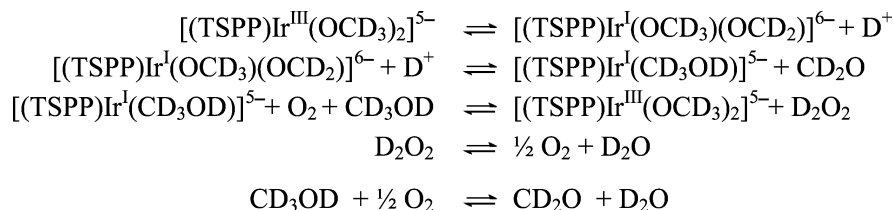
Scheme 2. Proposed Pathway for Methanol Reduction of Iridium(III) Porphyrins at High pD
