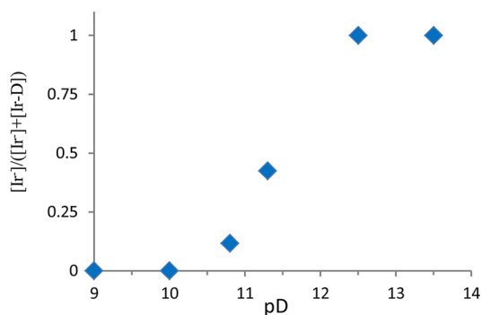
Figure 5. Acid dissociation constant for [(TSPP)Ir-D(CD 3 OD)] 4- in CD 3 OD from [(TSPP)Ir I (CD 3 OD)] 5- in equilibrium with the [(TSPP)Ir-D(CD 3 OD)] 4- as a function of pD from 1 H NMR. Nonlinear least-squares fit gives K_5(298\text{K}) = 3.5 \times 10^{-12} .
