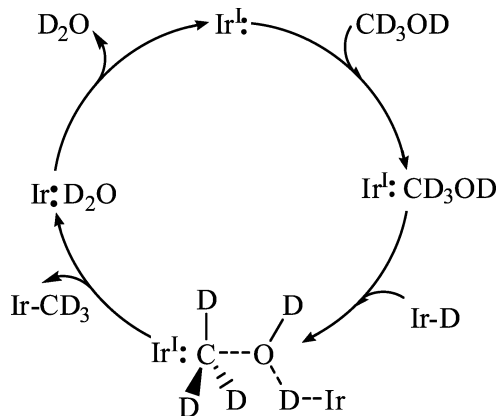
Scheme 3. Reaction of [(TSPP)Ir-D(CD 3 OD)] 4- and CD 3 OD To Form [(TSPP)Ir-CD 3 (CD 3 OD)] 4- and Water Catalyzed by [(TSPP)Ir I (CD 3 OD)] 5- in Methanol
