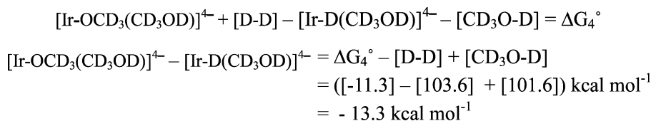
Scheme 5. BDFE of [(\text{Ir}-\text{OCD}_3)-(\text{Ir}-\text{D})] Derived from the Reaction of [\text{Ir}-\text{OCD}_3(\text{CD}_3\text{OD})]^{4-} and D 2
