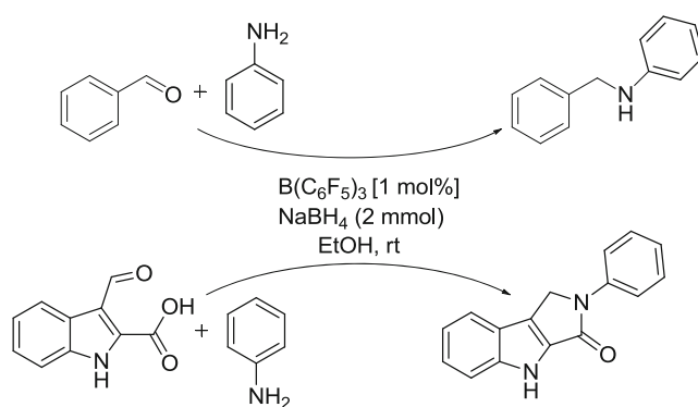
Scheme 1. B(C 6 F 5 )/NaBH 4 mediated synthesis of N -benzylaniline and 2-phenyl-1,2-dihydropyrrolo[3,4- b ]indol-3(4 H )-one.
