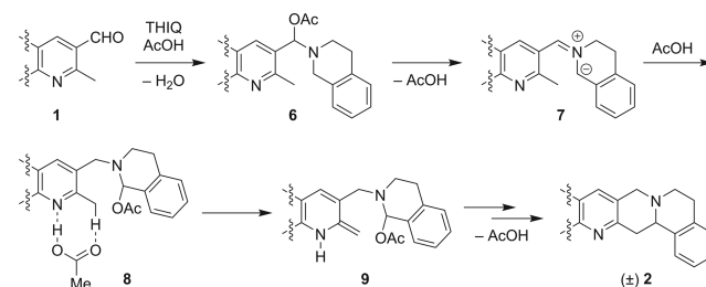
Scheme 4. Proposed Mechanism
