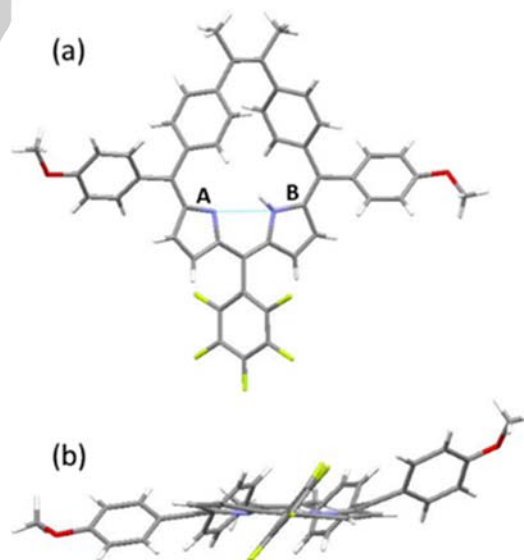
Figure 6. Top and side view of the molecular structure of compound 20 in the crystal.
