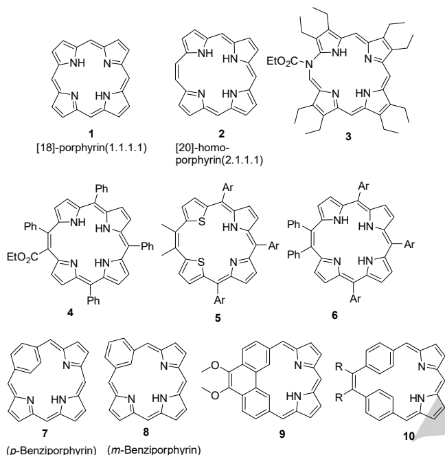
Figure 1. Fundamental structures of porphyrins, homoporphyrins, benziporphyrins and target systems.
