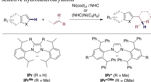
Scheme 1: Ligands and catalysts employed for the linear-selective hydroheteroarylation
