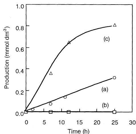
Figure 2. Electrochemical reduction of NADP + to NADPH at NADP + -dependent ALDH (a), and that of NAD + to NADH at NAD + -dependent ALDH obtained from Bakers Yeast (b) and obtained from Equine Liver (c). E = -0.85 V vs. Ag/AgCl.
