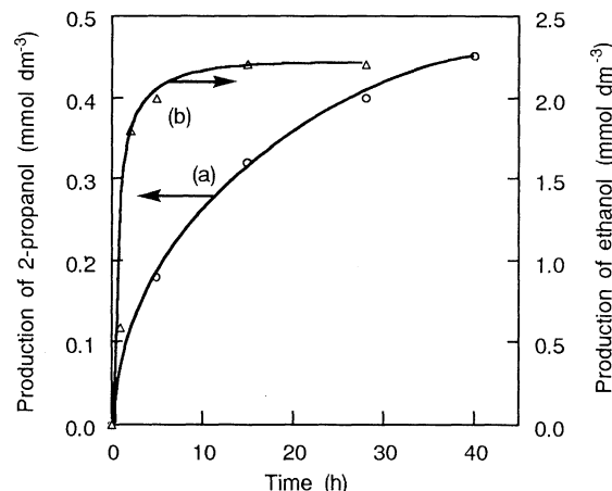
Figure 3. Electrochemical reduction of acetone to 2-propanol (a) and that of acetaldehyde to ethanol (b) using NADP + -dependent ALDH and NAD + -dependent ALDH as a bifunctional electrocatalyst, respectively, together with acetophenone as the product(1). E = -0.85 V vs. Ag/AgCl.
