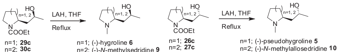
Scheme 11. Synthesis of (–)-N-methylsedridine and (–)-N-methylallosedridine.
