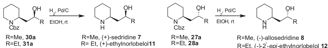
Scheme 10. Synthesis of sedridine and norlobelol.
