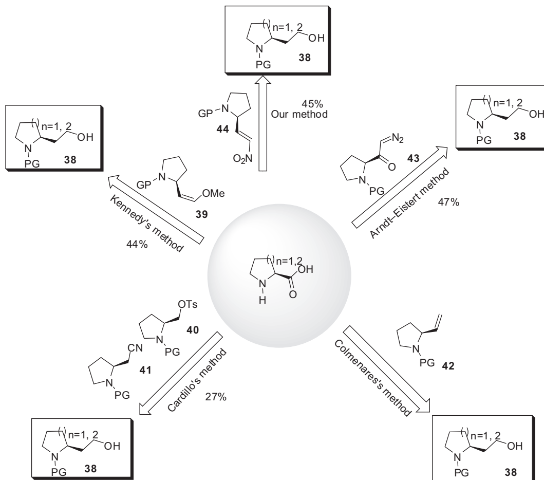
Scheme 12. Methods for one-carbon homologation of proline and pipecolic acid.
