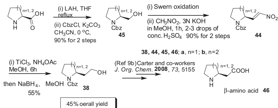
Scheme 13. Reductive Nef method for homologation of proline and pipecolic acid.
