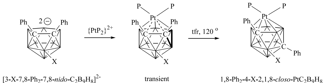
Scheme 1. Metallation of [3\text{-X-}7,8\text{-Ph}_2\text{-}7,8\text{-nido-C}_2\text{B}_9\text{H}_8]^{2-} with a \{\text{Pt(PMe}_2\text{Ph)}_2\}^{2+} fragment (abbreviated to \{\text{PtP}_2\}^{2+} for clarity) generating a 4-X-labelled C-atom isomerised 2,1,8-PtC 2 B 9 species via rotation of the (bold) CB 2 face of a notional 6-X-3,1,2-PtC 2 B 9 intermediate. Compound 1 corresponds to the intermediate and compounds 2 and 3 to the final product.
