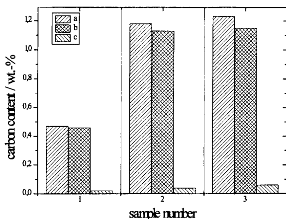
Fig. 3. Carbon content on the chromia surface under different conditions. Sample 1: chromia conditioned with CFC-12; sample 2: chromia conditioned with HFC-134 and then treated with CFC-12; sample 3: chromia conditioned with CFC-12 and then treated with HFC-134. The histograms correspond to (a) original samples; (b) samples a following evacuation at 400 °C; and (c) samples a following treatment with O 2 .
