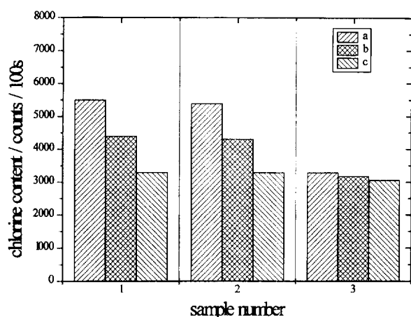
Fig. 2. Chlorine content on the chromia surface under different conditions. Sample 1: chromia conditioned with CFC-12; sample 2: chromia initially conditioned with HFC-134 and then treated with CFC-12; sample 3: chromia conditioned with CFC-12 and then treated with HFC-134. The histograms correspond to (a) the original samples; (b) samples a following evacuation at 400 °C; and (c) samples a following treatment with O 2 .
