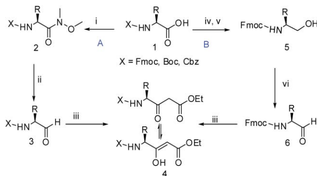
Scheme 1 Synthesis of N -protected \gamma -amino \beta -keto esters from the coupling reaction between amino aldehydes and ethyl diazoacetate in the presence of tin(II) chloride. Reagents and conditions: (i) HBTU, HOBT, DiPEA, HCl-NH(OMe)Me, 2 h, 93–97%; (ii) LAH, THF, 0 °C, 30 min, 86–92%; (iii) ethyl diazoacetate, DCM, 20 mol% SnCl 2 , 76–84%; (iv) isobutyl chloroformate, DiPEA, THF; (v) NaBH 4 , H 2 O, 90–98%; (vi) Dess–Martin periodinane, DCM, 84–95%.
