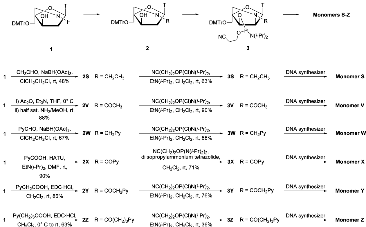
SCHEME 1. Synthesis of N2'-Functionalized 2'-Amino- \alpha -L-LNA Phosphoramidites a
