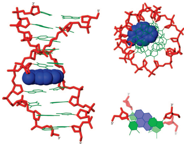
FIGURE 7. Three representations of the lowest energy structure of W2:D2 ; side view (left), top view (upper right), and truncated top view showing W5A6:T13A14 (lower right). Coloring scheme as in Figure 3 except that pyren-1-yl-methyl moiety of monomer W is in blue.
