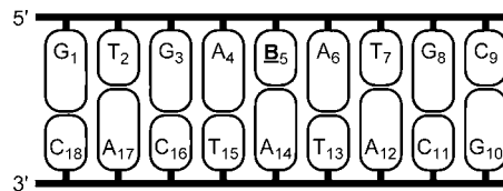
FIGURE 4. Nucleotide numbering for duplexes studied by molecular modeling; B = thymine (D1) or monomers O–Z (O2–Z2).
