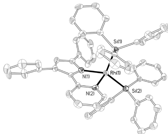
Figure 3. ORTEP diagram of the X-ray crystal structure of 9 ; the metal hydrides were not located from the difference Fourier map. Hydrogen atoms are omitted for clarity. Bond lengths (Å) and angles (deg): Rh1–N1 = 2.039(4), Rh1–N2 = 2.154(5), Rh1–Si1 = 2.318(2), Rh1–Si2 = 2.339(2), ∠N1–Rh1–N2 = 78.0(1), ∠Si1–Rh1–Si2 = 115.00(6), ∠N1–Rh1–Si1 = 106.6(1), ∠N1–Rh1–Si2 = 136.0(1), ∠N2–Rh1–Si1 = 100.3(1), and ∠N2–Rh1–Si2 = 107.2(1).
