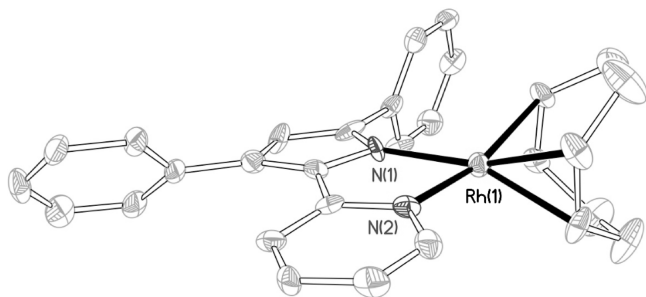
Figure 1. ORTEP diagram of the X-ray crystal structure of 4 . Hydrogen atoms are omitted for clarity. Bond lengths (Å) and angles (deg): Rh1–N1 = 2.079(7), Rh1–N2 = 2.094(7), \angle N1–Rh1–N2 = 79.1(3).
