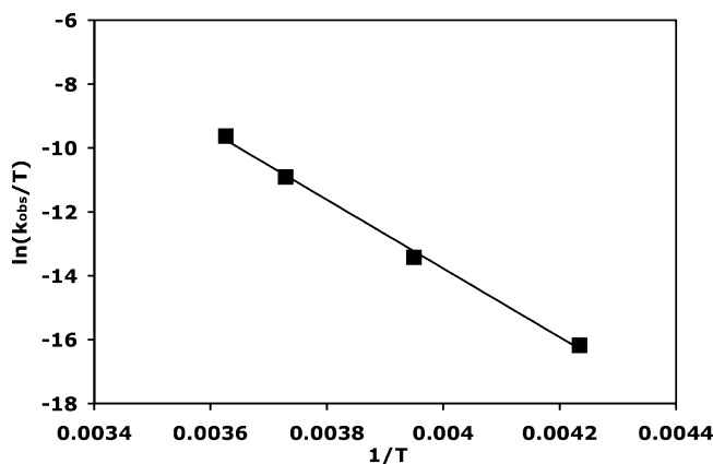
Figure 7. Eyring plot for the conversion of 10 to (\text{PyPyr})\text{Rh}(\text{H})_2(\text{Si}^i\text{BuPh}_2)(\text{SiEt}_3) .
