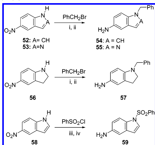
Scheme 8 a
