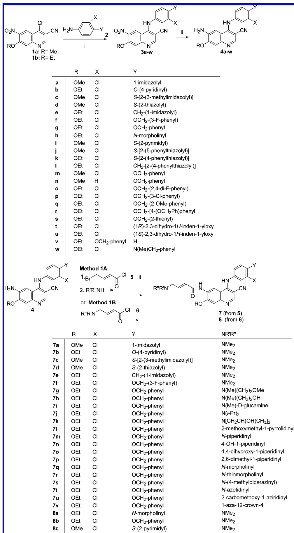
Scheme 1. Methods 1A and 1B a
