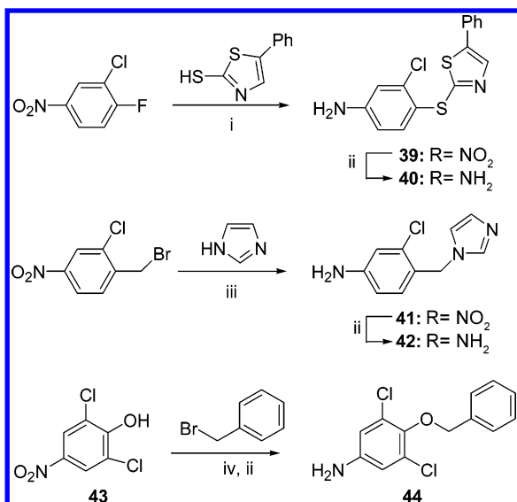
Scheme 6 a
