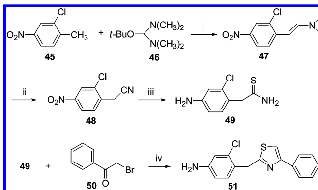
Scheme 7 a
