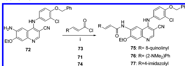
Scheme 11 a
