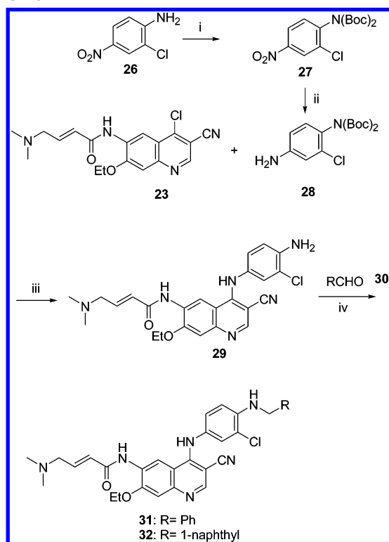
Scheme 4 a
