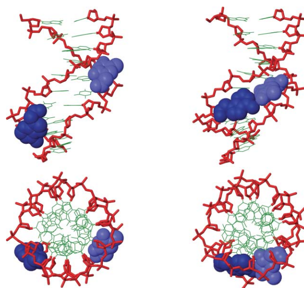
Fig. 2 Illustrations of the lowest energy structures of doubly modified duplex 5'-GTG AA T T T AGC C:3'-CAC TTA T A A CG G, without (to the left) and with forced hydrogen bonding of the extra nucleobases, respectively. Coloring scheme: nucleobases: green; sugar-phosphate backbone: red; N2'-thymin-1-ylacetyl: light blue; N2'-adenin-9-ylacetyl: blue.
