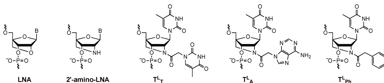
Fig. 1 LNA, 2'-amino-LNA and “double-headed” 2'-amino-LNAs.
