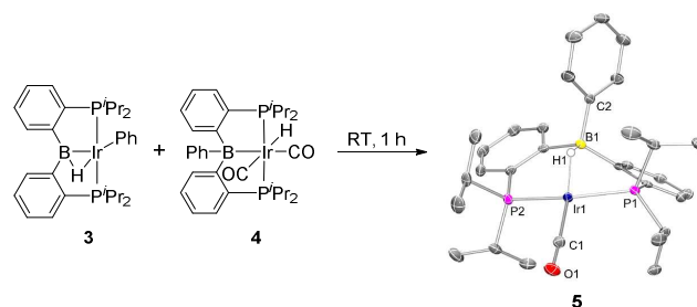
Scheme 2. Synthesis of 5 by comproportionation of 3 with 4 . a
