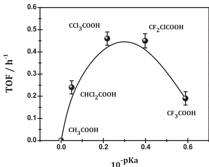
Fig. 2. Effect of proton concentrations on the Diels-Alder and dehydration reactions of DMF with ethylene to produce p -xylene. Reaction conditions: 5 mL 0.2 M DMF in dioxane, 0.1 mmol catalyst, T = 473 K, t = 4 h, P = 3.5 MPa ethylene.
