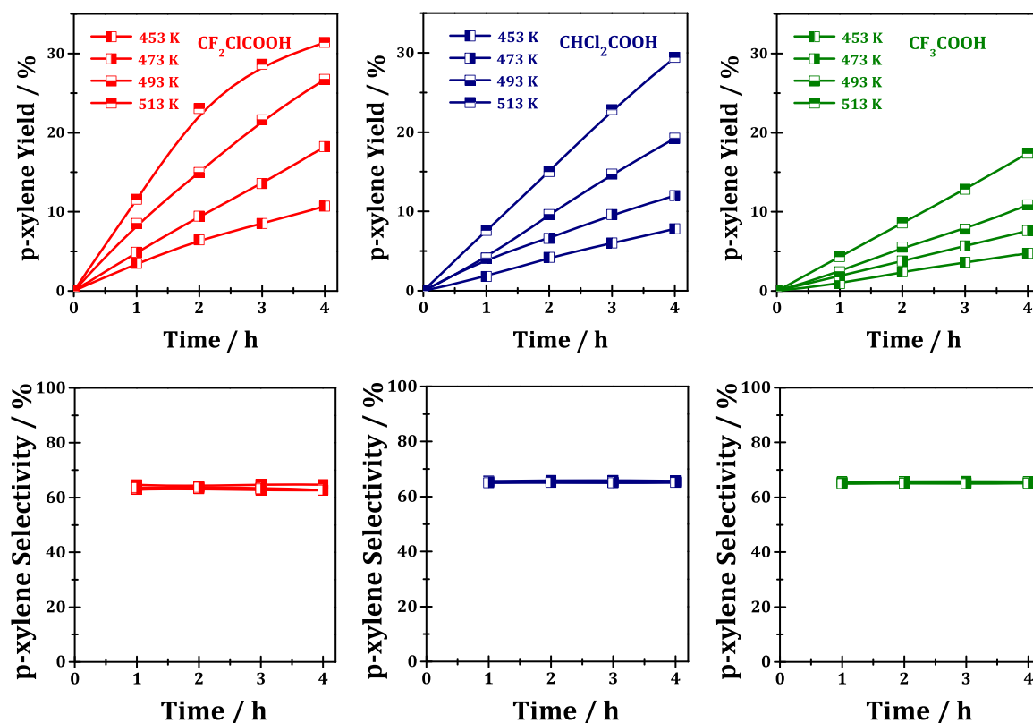
Fig. 3. Kinetics of the Diels-Alder and dehydration reactions of DMF with ethylene over haloacetic acid catalysts. Reaction conditions: 5 mL 0.2 M DMF in dioxane, 0.1 mmol catalyst, T = 453\text{K}–513 K, P = 3.5 MPa ethylene.
