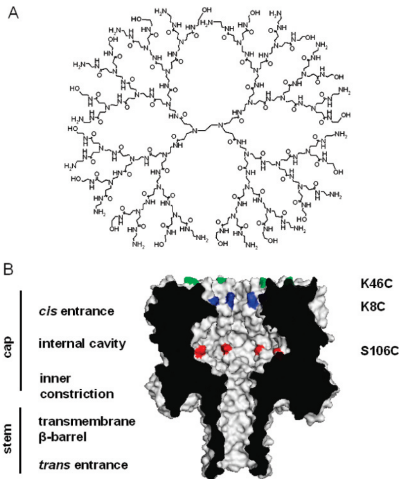
Figure 1. (A) Structure of a poly(amidoamine) dendrimer of generation 3 with 50% amine and 50% hydroxyl terminal groups. (B) Cross-sectional view of the heptameric \alpha HL pore with cysteine substitutions K46C, K8C, and S106C. The model was generated using crystallographic data 13 and PyMol. The internal diameters of the channel are as follows: 2.9 nm, cis entrance; 4.1 nm, internal cavity; 1.3 nm, inner constriction; 2 nm, trans entrance of the \beta -barrel.
