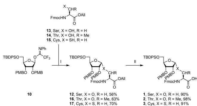
Scheme 2. Synthesis of Fmoc-based SPPS building blocks 1–3. Reagents and conditions: I) TBSOTf, acceptors 13, 14 or 15, DCM, –50 °C. II) Pd(PPh 3 ) 4 , DMBA, DCM. All = allyl.
