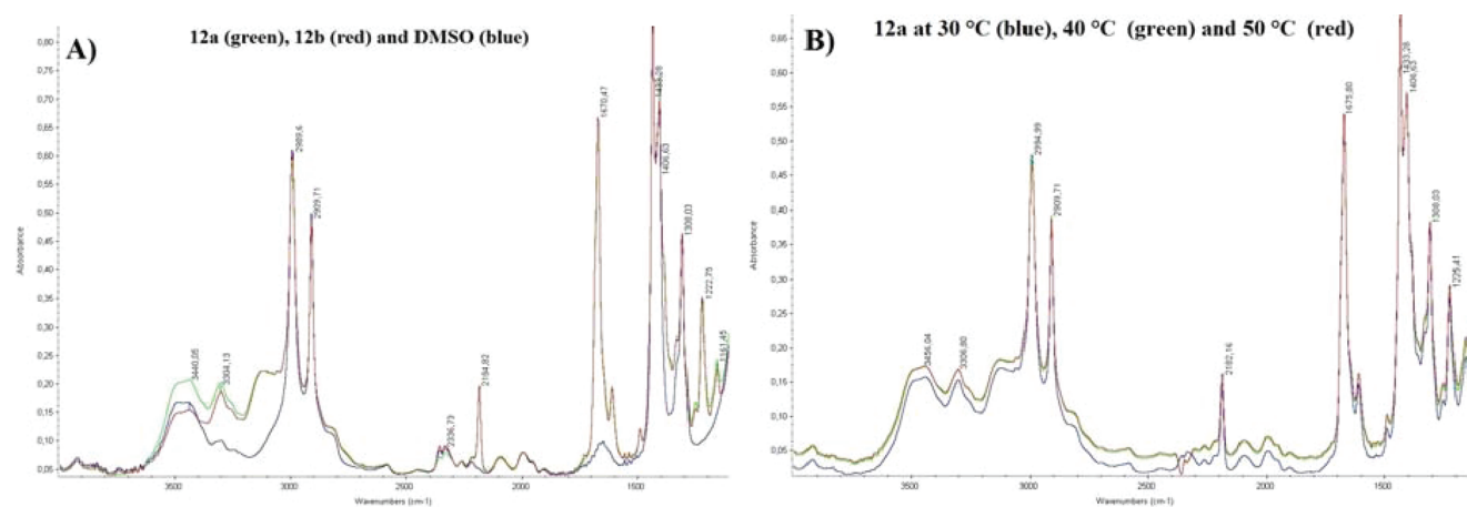
Figure 8. Experimentally determined IR spectra of 12a and 12b in DMSO using a FTIR apparatus. (A) IR spectra at rt of 12a (green) and 12b (red) at 8 cm -1 resolution (20 min) in DMSO (blue) solution (150 mg/mL) using a CaF 2 cell and 6 μm spacer. (B) IR spectra of 12a at 30 °C (blue), 40 °C (green) and 50 °C (red).
