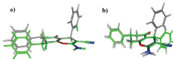
Figure 3. Superimposition of low-energy conformations of 1. (a) Stereochemistry at C4 (R 2 ) is conserved: syn -isomer (green) and anti -isomer (gray); (b) stereochemistry at C7 (R 1 ) is conserved: syn -isomer (green) and anti -isomer (gray).
