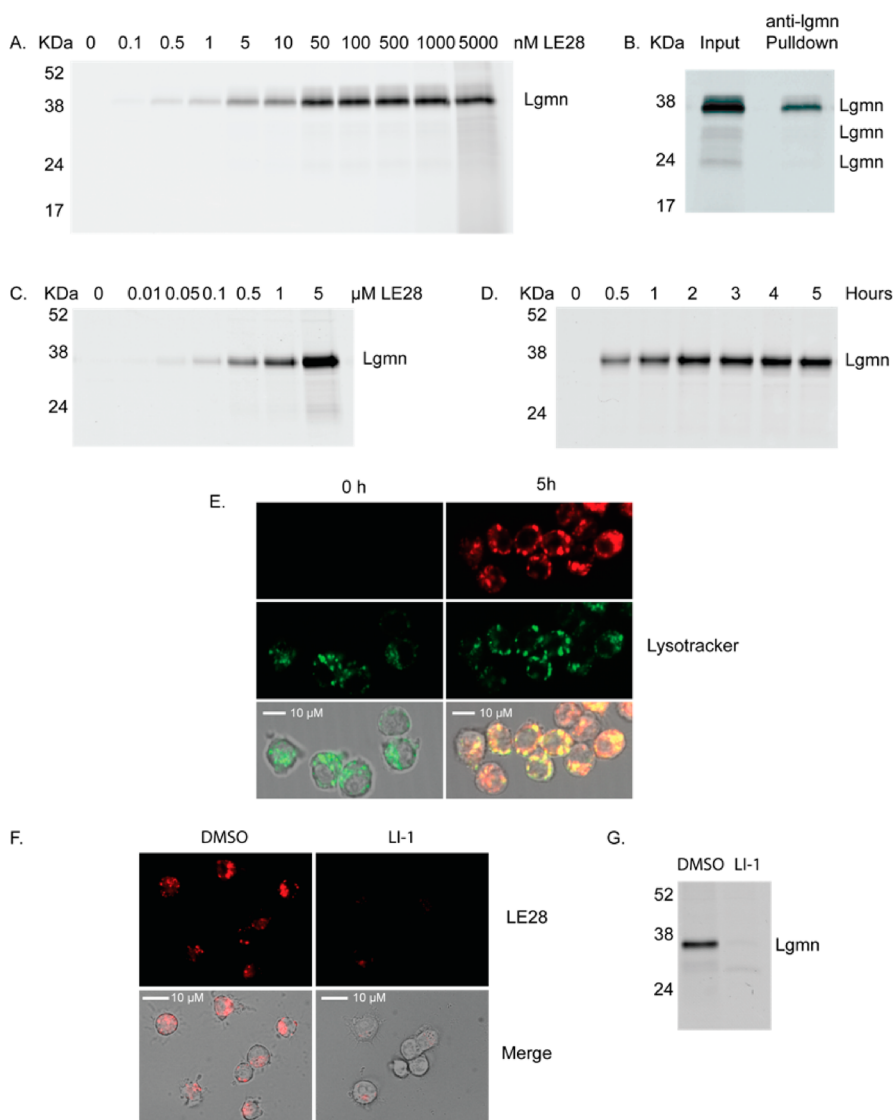
Figure 2. (A) Fluorescent SDS-PAGE showing dose-dependent labeling of legumain by LE28 in RAW cell macrophage extracts. (B) Immunoprecipitation of LE28-labeled RAW cell lysates using a legumain-specific polyclonal antibody. (C) RAW cells were labeled at the indicated dose of LE28 for one hour followed by lysis and fluorescent SDS-PAGE. (D) RAW cells were incubated with 1 μM LE28 for the indicated time period followed by lysis and fluorescent SDS-PAGE. (E) Microscopy images of RAW cells exposed to LE28 (red) for 0 or 5 h. Lysotracker (green) was used to reveal the location of lysosomes. (F) Microscopy of RAW cells exposed to DMSO vehicle or 100 μM of the legumain inhibitor, LI-1 followed by incubation with LE28. (G) SDS-PAGE analysis of RAW cells exposed to DMSO vehicle or LI-1, followed by labeling with LE28.
