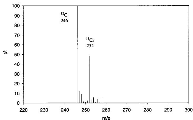
Figure 1. Molecular ion region from the electron impact mass spectrum of [ ^{14}\text{C} -UL-phenyl]-[ ^{13}\text{C}_6 -phenyl]-O-ethyl-S-phenylethyl-phosphonodithioate.
