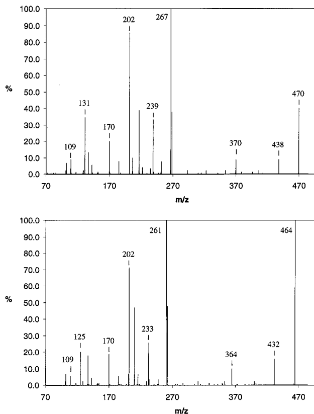
Figure 3. CID spectra of m/z 470 (top) and 464 (bottom) from the LC-MS-MS analysis of methylated metabolite A15.
