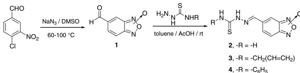
Scheme 2. Synthesis of thiosemicarbazone-benzofuroxan hybrid derivatives 2–4 .
