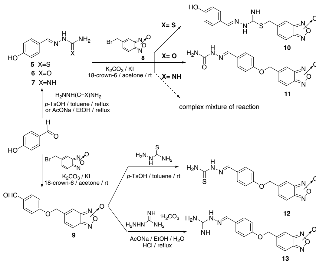
Scheme 3. Synthesis of semicarbazone-, thiosemicarbazone-, and amidinohydrazone-benzofuroxan hybrid derivatives.
