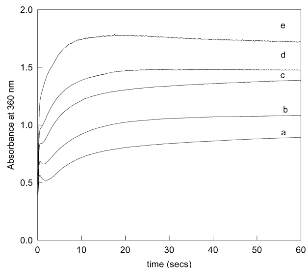
Figure 3. Variation of [ClO_2^-] in cysteine oxidation by chlorite spanning chlorite/cysteine ratios of 4.0 to 7.0. High ratios show a monotonic increase in chlorine dioxide without a transient peak. [cysteine]_0 = 5 \times 10^{-3} M , I = 1.0 M . [ClO_2^-] = (a) 0.02 M, (b) 0.025 M, (c) 0.0275 M, (d) 0.03 M, (e) 0.035 M.
