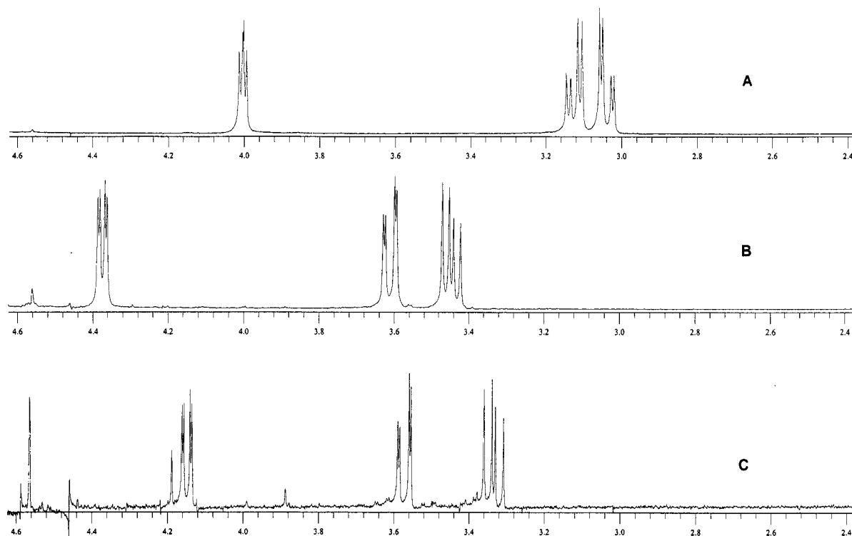
Figure 1. (A) NMR spectrum of L-cysteinesulfinic acid in nearly neutral acidic conditions. It shows the expected split doublet from protons H_B and H_C and the triplet from proton H_A . Each integrates as a single proton. (B) Spectrum from the products of cysteine and chlorite. Assignment: H_A (4.0 ppm); H_B (3.04 ppm); H_C 3.12 ppm). It shows basically the same spectrum as in A shifted slightly downfield due to the formation of the sulfonic acid which accompanies the oxidation of cysteine. The relative assignments with respect to field for protons H_A , H_B , and H_C in spectrum A remain unchanged. The larger coupling constants can be attributed to the larger sulfonic acid group which renders protons H_B and H_C more dissimilar. (C) NMR spectrum of the product of cysteinesulfinic acid with excess chlorite. The spurious peaks represent impurities produced in the synthesis of the cysteinesulfinic acid (Fisher Scientific). However, both spectra show that there is no change in the carbon backbone. These spectra were also indistinguishable from that of cysteic acid.
