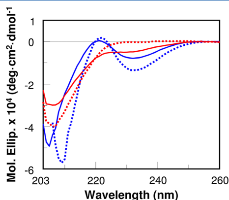
Figure 3. CD spectra of SolyC2 (blue) and SolyC2-ox (red) (50 \mu M) recorded in 10 mM phosphate buffer pH 7 (continuous line) and in 10 mM phosphate buffer, 30 mM SDS pH 7 (dotted lines).
