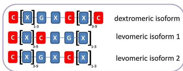
Figure 1. Schematic representation of the gamma core isoforms.
