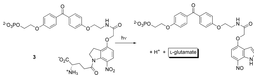
FIGURE 2. Expected photolytic reaction pathway for 3 , showing release of L-glutamate.
