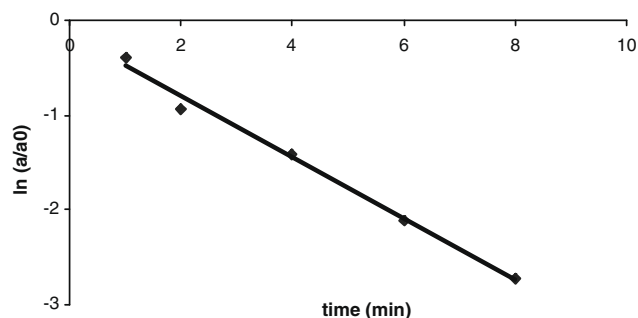
Figure 2. A representative plot for the disappearance of 2 in the presence of thiol. Compound 2 (2.5 \mu L of a 10 mM stock in \text{CH}_3\text{CN} ) was added to a mixture containing sodium phosphate buffer (50 \mu L, 500 mM, pH 7.0), water (150 \mu L), 2-mercaptoethanol (50 \mu L of a 10 mM stock) and acetonitrile (247.5 \mu L) at 25 ^\circ\text{C} . The mixture (final concentrations: 2 , 50 \mu\text{M} ; buffer, 50 mM, pH 7.0; thiol, 1 mM; acetonitrile, 50% by volume) was vortex mixed and the disappearance of 2 (a is the peak area at time = t and a_0 is the peak area at time = 0) monitored by reverse phase HPLC at regular time intervals as described in the legend for Figure 1. From the slope of the plot, a pseudo-first-order rate constant of 5.5 \times 10^{-3} \text{ s}^{-1} ( t_{1/2} = 2 \text{ min} ) at 1 mM thiol was obtained. This corresponds to an apparent second-order rate constant of 5.5 \pm 0.2 \text{ M}^{-1} \text{ s}^{-1} .
