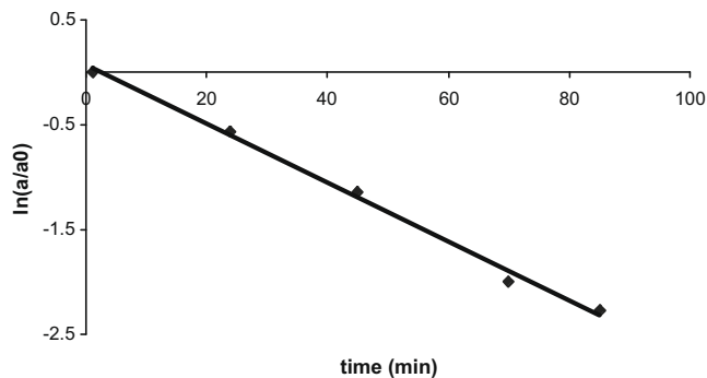
Figure 3. Representative plot for the disappearance of 2 in the absence of thiol. Compound 2 (2.5 \mu L of a 10 mM stock in \text{CH}_3\text{CN} ) was incubated at 25 ^\circ\text{C} in a solution composed of sodium phosphate buffer (50 \mu L, 500 mM, pH 7.0), water (200 \mu L) and acetonitrile (247.5 \mu L). The mixture (final concentrations: 2 , 50 \mu\text{M} ; buffer, 50 mM, pH 7.0; acetonitrile, 50% by volume) was vortex mixed and the disappearance of compound 2 (a is the peak area at time = t and a_0 is the peak area at time = 0) analyzed by reverse phase HPLC as described in the legend of Figure 1. The pseudo-first-order rate constant of 0.027 \pm 0.001 \text{ min}^{-1} was obtained from the slope of the plot. This corresponds to a half-life of 26 min for the hydrolysis of 2 under these conditions.
