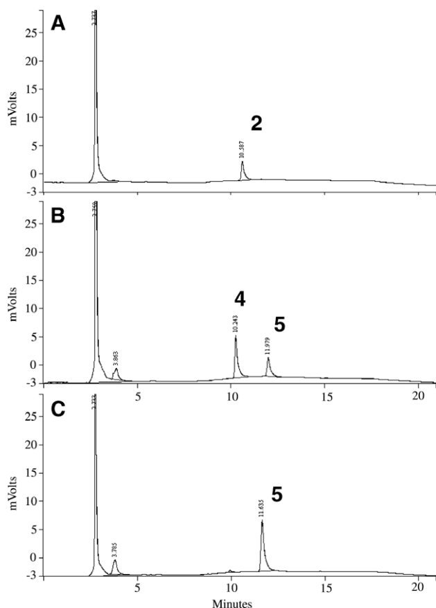
Figure 1. Reaction of 2 with 10 equiv 2-mercaptoethanol in aqueous buffer: (A) Compound 2 alone in buffer, (B) 1 min after addition of thiol, (C) 25 min after addition of thiol. Compound 2 (2.5 \mu L of a 10 mM stock in \text{CH}_3\text{CN} ) was added to a mixture containing sodium phosphate buffer (50 \mu L, 500 mM, pH 7.0), water (275 \mu L), 2-mercaptoethanol (25 \mu L of a 10 mM stock in water), and acetonitrile (147.5 \mu L) at 25 ^\circ\text{C} (final concentrations: 2 , 50 \mu\text{M} ; buffer, 50 mM, pH 7.0; thiol, 500 \mu\text{M} ; acetonitrile, 30% by volume). The disappearance of 2 was monitored at 254 nm. Aliquots (40 \mu L) from the reaction mixture were injected onto a C-18 Varian Microsorb–MV column, 100 \text{\AA} sphere size, 5 \mu\text{m} pore size, 25 cm length, 4.6 mm i.d. eluted with a solvent system composed of water with 0.5% acetic acid v/v (A) and acetonitrile (B), at a flow rate of 0.8 mL/min. The column was eluted with 70:30 A/B for 4 min and then ramped to 50:50 A/B over 4 min, held at 50:50 A/B for 7 min, and then ramped back to 70:30 A/B over the next 3 min. The peak at 10.2 min was identified as the mixed disulfide 4 . The identity of 4 was confirmed by co-injection with an authentic standard 22 and by LC/MS analysis which showed that the compound displays an m/z of 316 corresponding to that expected for the [\text{M}+\text{H}]^+ ion of 4 . The early peaks in the chromatogram correspond to buffer salts, 2-mercaptoethanol, and the disulfide of 2-mercaptoethanol.
