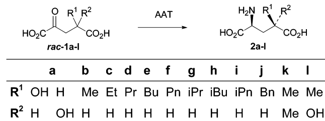
SCHEME 1. AAT-Catalyzed Synthesis of Glutamic Acid Analogues
