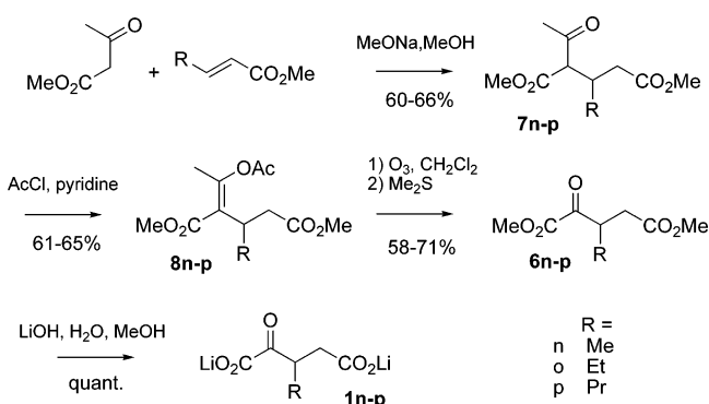
SCHEME 3. Synthesis of KG Analogues by Ozonolysis of Enol Acetates
