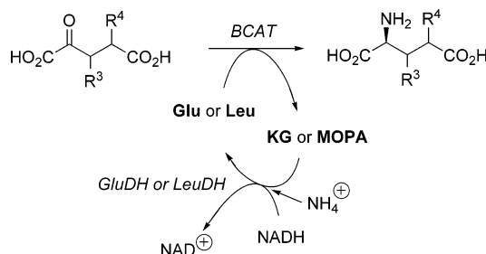
SCHEME 4. BCAT Activity Assay
