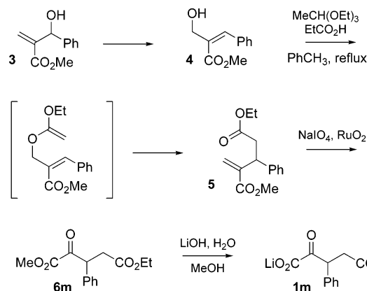
SCHEME 3. Synthesis of KG Analogues by Ozonolysis of Enol Acetates
