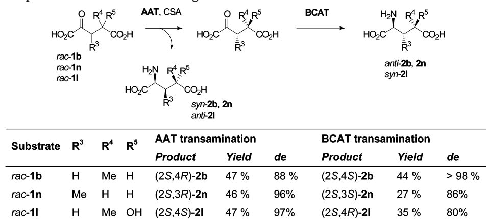
SCHEME 7. Two-Step Transamination Process Using AAT and BCAT
