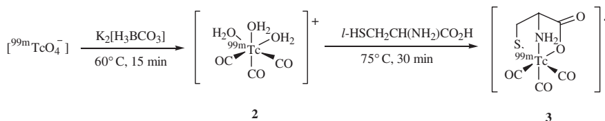
Scheme 2. Preparation of 99m Tc(I) tricarbonyl cysteine complex ( 3 )
