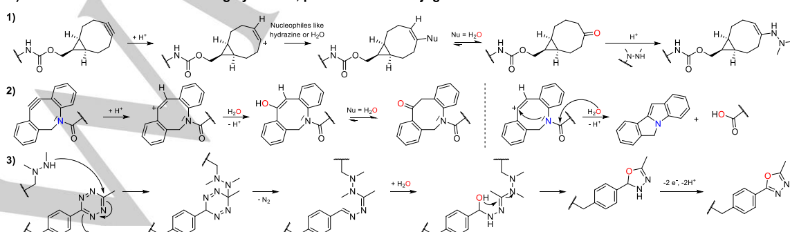
Scheme 2. Bifunctional HIPS reagents and observed side reactions. A) Two step synthesis (coupling and deprotection) of HIPS-CF ( 2 ), -mTet ( 3 ), -DBCO ( 4 ), -BCN ( 5 ), and -azide ( 6 ). B) Postulated side reactions during synthesis, purification or conjugation. 1) Postulated acid-mediated decomposition of BCN. 2) Possible mechanism for proton catalyzed decomposition of DBCO. 3) Observed inter- or intramolecular hydrazine catalyzed decomposition of HIPS-mTet ( 3 ).
