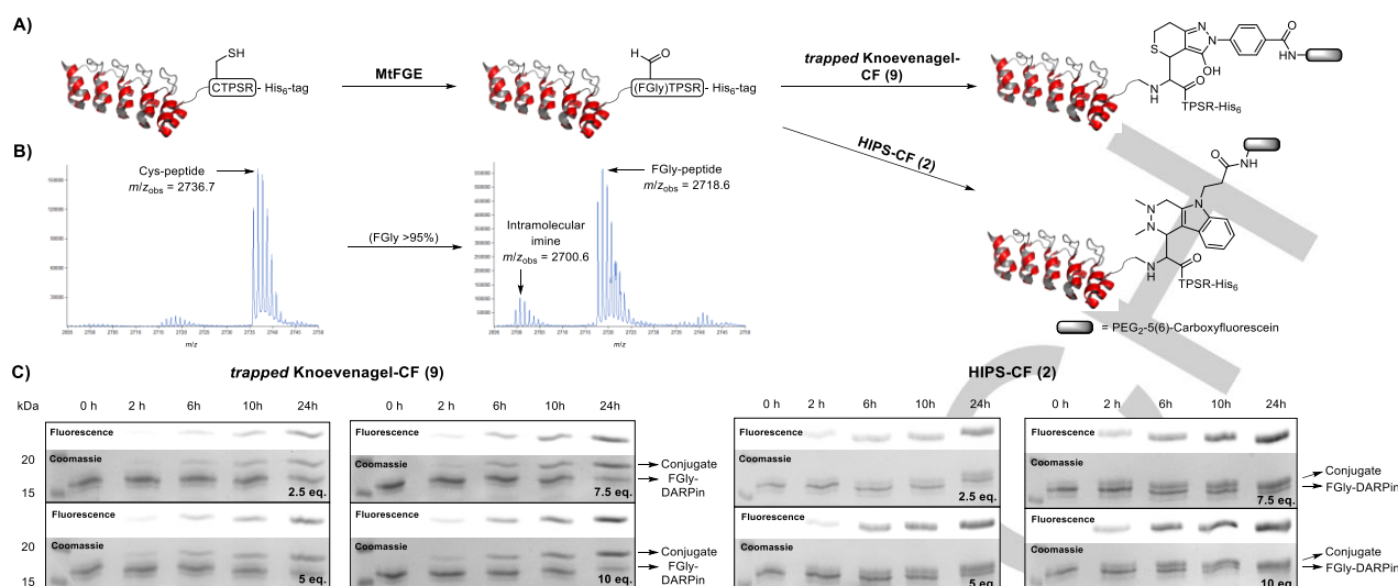
Figure 1. Stoichiometry- and time-dependent conjugation assay with HIPS-CF ( 2 ) and trapped Knoevenagel-CF ( 9 ). A) Bioconjugation experiments: DARPIn-CTPSR-His 6 (100 \mu M) was enzymatically oxidized in a bicine buffer containing 10 mol% CuSO 4 and 10 mol% CTPSR-MtFGE. The FGly-containing DARPIn was re-buffered (HIPS: 100 mM phosphate, 30 mM NaCl, pH 6.0; Knoevenagel: 50 mM citrate, 50 mM NaCl, pH 7.2) and subsequently fluorescence labeled using 2 and 9 (30 \mu M FGly-DARPIn). B) MALDI-ToF analysis of relevant Cys- ( m/z = 2736.6) and FGly-peptide ( m/z = 2718.6 and 2700.6). C) SDS-PAGE analysis (15%) of stoichiometry- (2.5, 5, 7.5 and 10 eq.) and time-dependent conjugation assays. Samples (15 \mu g) were taken at 2, 6, 10 and 24 hours and analyzed on gel by fluorescence (upper panels) before Coomassie staining (lower panels). Whole SDS gels and fluorescence images can be found in the SI (Fig. S12 and S13).
