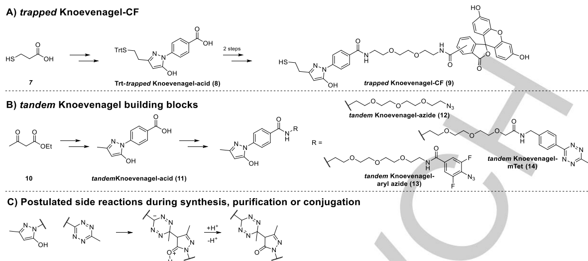
Scheme 3. Bifunctional Knoevenagel reagents and observed side reactions during synthesis, purification or conjugation. A) Synthesis of trapped Knoevenagel-CF (9) starting from 3-mercaptopropionic acid (7). B) Synthesis of tandem Knoevenagel-azide (12), fluorine substituted aryl azide (13) and -mTet (14). C) Postulated inter- and intramolecular side reaction of pyrazolone with methyl substituted tetrazine.
