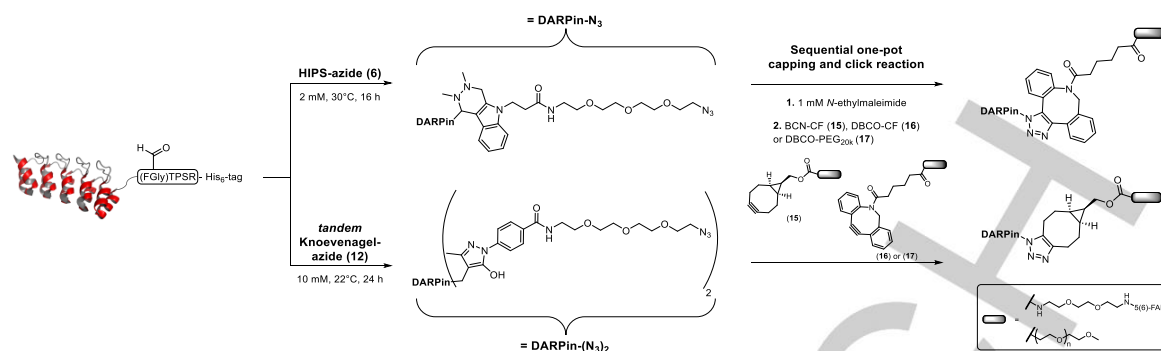
Scheme 4. Azide-derivatization of DARPin by HIPS-azide ( 6 ) and tandem Knoevenagel-azide ( 12 ). FGly-DARPin was first conjugated with HIPS-azide ( 6 , 2 mM, 16 h, 30°C) or tandem Knoevenagel-azide ( 12 , 10 mM, 24 h, 22°C), rebuffed in phosphate buffer (100 mM phosphate, 150 mM NaCl, pH 7.2, 8% DMSO) and then used in a sequential one-pot capping and click reaction with different strained alkynes.
