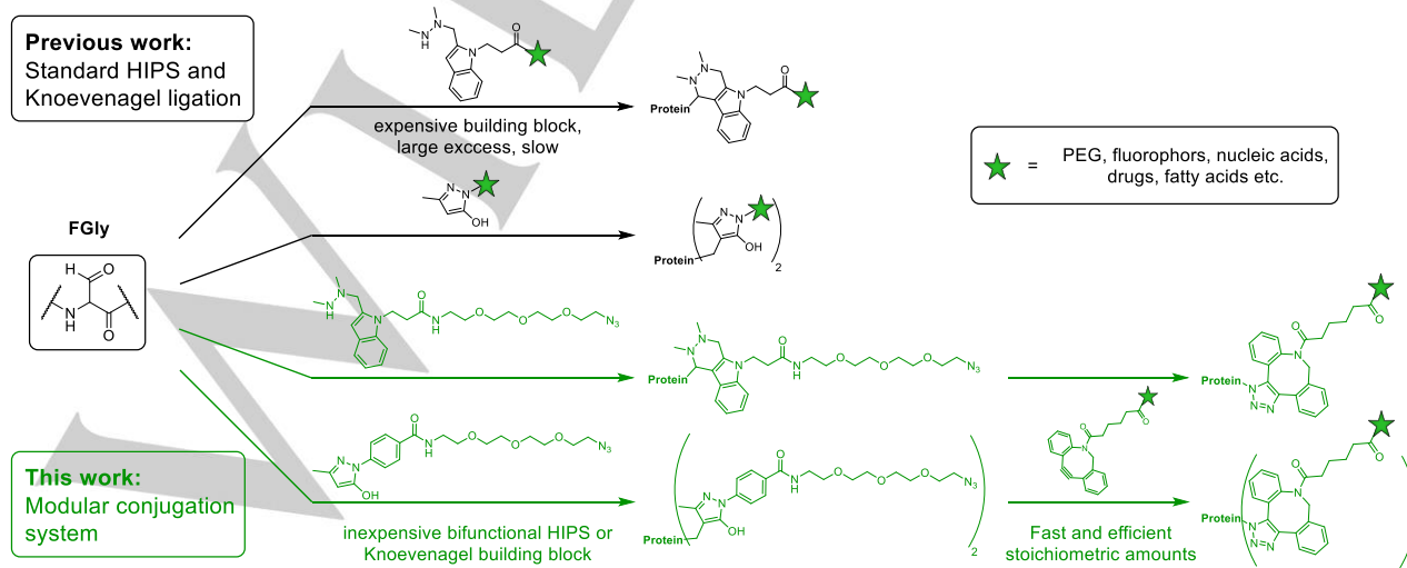
Scheme 1. Development of a highly efficient modular conjugation system for mono- and double-conjugation using stoichiometric amounts of DBCO-derivatives.
