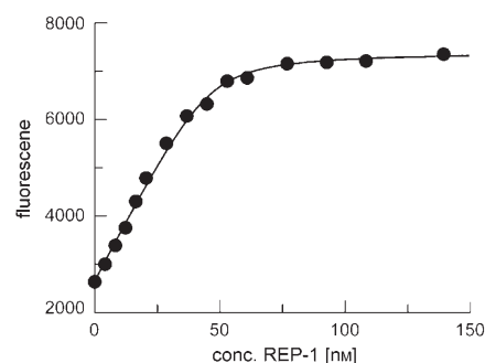
Figure 5. Spectrofluorometric titration of 19a with REP-1. Conditions: 25°C, 25 mM HEPES pH 7.2, 40 mM NaCl, 2 mM MgCl_2 , 2 mM DTE and 20 \mu M GDP. The concentrations of 19a complexes were 50 nM. The excitation/emission wavelengths were fixed at 333/440 nm. Data were fitted to a quadratic equation as implemented in the program Grafit 5.1 (Eritacus software) leading to K_d value of 1.9 \pm 0.5 nM and consistent with 1:1 stoichiometry. DTE: dithioerythritol, HEPES: 2-[4-(2-hydroxyethyl)-1-piperazinyl]ethanesulfonic acid.
