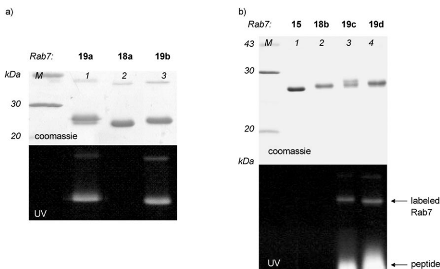
Figure 4. SDS-PAGE analysis of the Diels–Alder ligation between masked Rab7 hexadienyl ester 18 and male-imide probes 6e and 12 . Diels–Alder labeled Rab7 19a–d appeared as a unique fluorescent protein band at ca 24 kDa. Ligation conditions: 18a and 100-fold 6e (lane 1 in a), 18a and 100-fold 12 (lane 3 in a), 18b and 50-fold 6e (lane 3 in b), 18b and 100-fold 12 (lane 4 in b).
