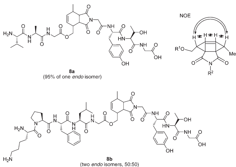
Figure 2. Structures of cycloadducts 8a and 8b .
