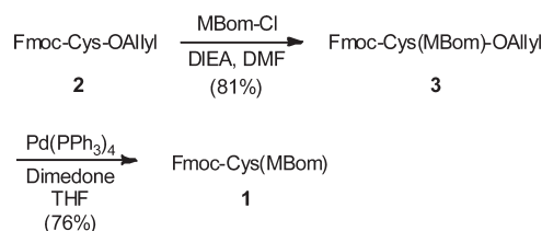
Scheme 1. Synthesis of Fmoc-Cys(MBom) ( 1 )
