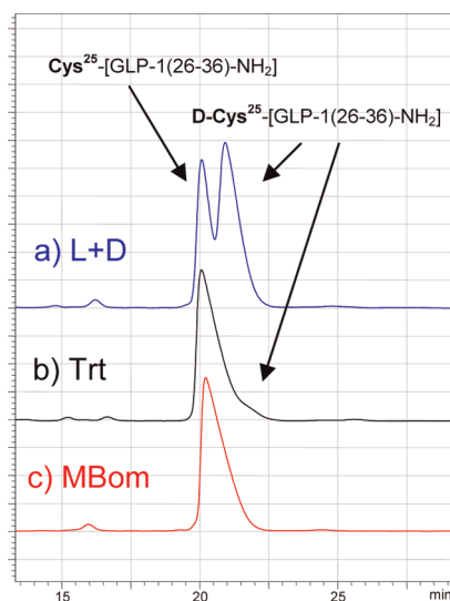
Figure 4. HPLC profiles of Cys 25 -[GLP-1(26–36)-NH 2 ]. (a) A mixture of L-Cys 25 - and D-Cys 25 -[GLP-1(26–36)-NH 2 ]. The product obtained by using Fmoc-Cys(Trt) (b) or Fmoc-Cys(MBom) (c). HPLC conditions are described in the Supporting Information.
