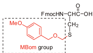
Figure 1. Structure of Fmoc-Cys(MBom) ( 1 ).
