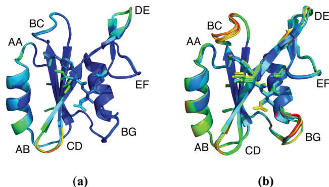
Figure 10. Adjusted atomic b-factors in complexes of the Grb2 SH2 domain (residues 59–151) with flexible and constrained ligands. Backbone atoms of residues are color-coded from blue to green to red for atoms having values of 20, 30, and 40 Å 2 . (a) Complexes of flexible ligands 5 , 6 , and 8 . (b) Complexes of constrained ligands 11 , 12 , and 14 .
