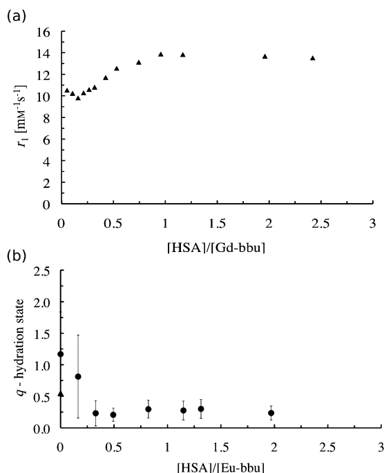
Figure 4. a) Relaxivity at 37°C, 0.47 T, pH 5, for Gd-bbu (0.42 mM) as a function of added HSA. b) Hydration number q of Eu-bbu at pH 5 as a function of added HSA. At [\text{HSA}]/[\text{Eu-bbu}]=0 ; \blacktriangle : measurements made on a visible aggregate; \bullet : measurements made on the supernatant.
