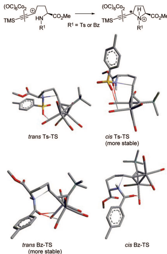
Figure 2. Geometries of the optimized transition states (hydrogens were omitted by clarity) for the cyclization to protonated 1c and 1d . Red thinner lines denote electrostatic interactions between the carbonyl group of the cobalt complex and the oxygens of the sulfonamide and benzamides groups.
