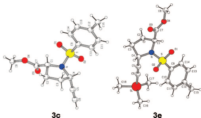
Figure 1. X-ray crystallographic structures of cis - and trans -tosylpyrrolidines 3c and 3e .
