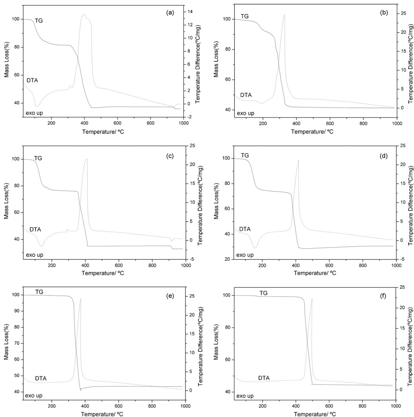
Fig. 4. Simultaneous TG–DTA curves of the compounds: (a) \text{MnL} \cdot 2\text{H}_2\text{O} ( m = 7.198 mg), (b) \text{FeL} \cdot \text{H}_2\text{O} (7.042 mg), (c) \text{CoL} \cdot 3\text{H}_2\text{O} (7.019 mg), (d) \text{NiL} \cdot 3\text{H}_2\text{O} (7.105 mg), (e) \text{CuL} (7.056 mg) and (f) \text{ZnL} (7.085 mg).
