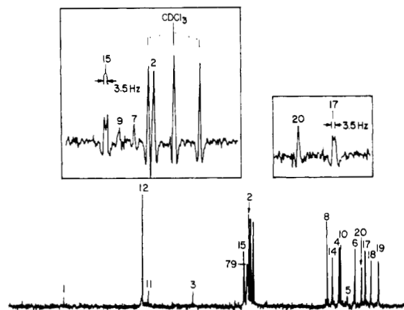
Figure 1. Carbon-13 NMR spectrum of aplasmomycin derived from [1,3-^{13}\text{C}_2] glycerol. Inserts: Scale expansions of the regions showing the C-15 and C-17 signals.
