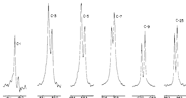
Figure 2. Partial ^{13}\text{C} NMR spectra of monensin A sodium showing the signals of carbons bearing oxygen-18. C-1, C-3, and C-5 signals are from monensin derived from [1-^{13}\text{C}, 1-^{18}\text{O}_2] propionate. C-7, C-9, and C-25 signals are from monensin derived from [1-^{13}\text{C}, 1-^{18}\text{O}_2] acetate. (Line broadening, -1.0 Hz; Gaussian multiplier, 0.3 Hz). Acquisition parameters are given in Table II.
