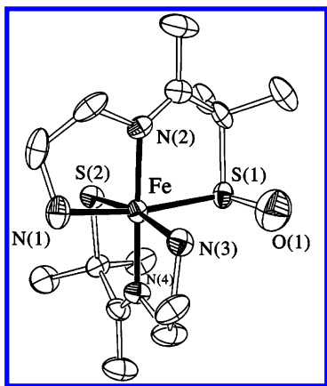
Figure 2. ORTEP diagram of the cation of [\text{Fe}^{\text{III}}(\text{ADIT})(\text{ADIT-O})]\text{Cl} \cdot \text{MeCN} \cdot \text{PhS}(\text{O})_2\text{NH}_2 ( 5a ), showing atom labeling scheme. All hydrogen atoms have been omitted for clarity.
