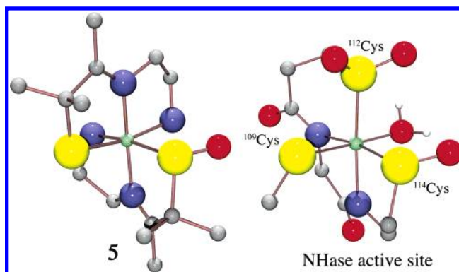
Figure 16. Comparison of the iron coordination environment of 5 with that of the NHase active site.
