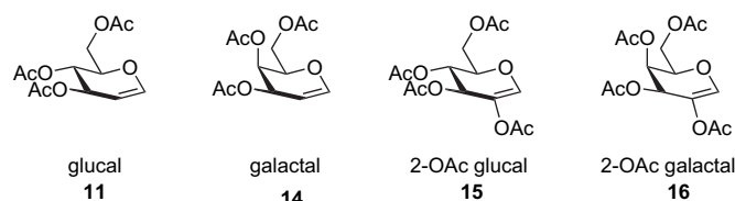
Figure 1. Glycal acceptors for the Ferrier reaction.
