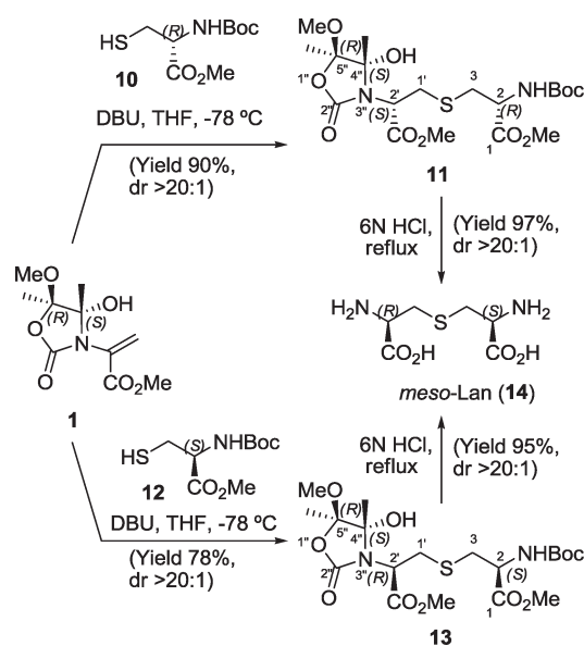
Scheme 2. Synthesis of meso -Lanthionine
